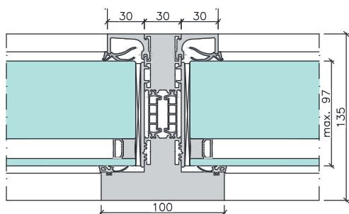
› Horizontal section B - B (Mullion)
