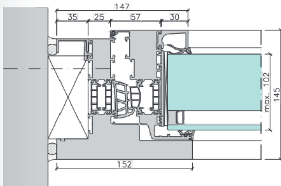
› Horizontal section A - A (Wall connection)
